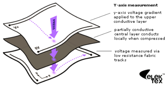
Figure 1. Pressure and position sensor.
