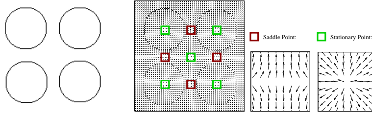
Figure 2: The four-disc problem - from left: An image contains four disc boundaries, the GGVF velocity map, enlarged saddle point (red square) and stationary point (green square).
